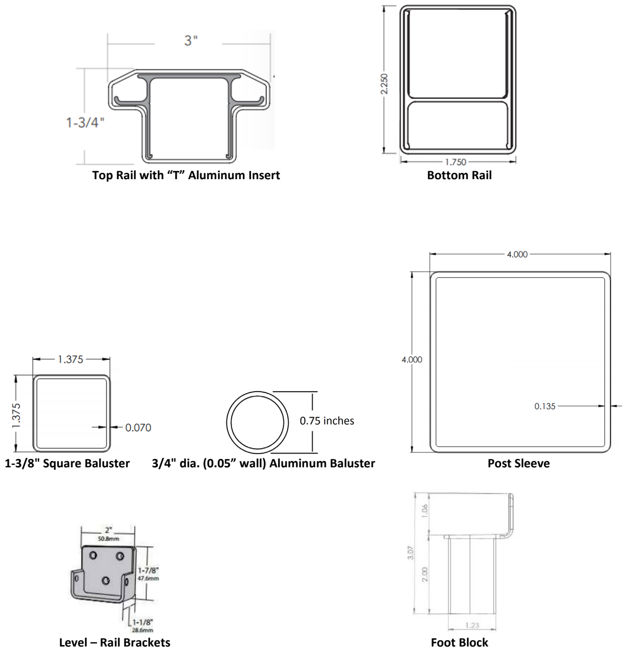
FIGURE 1 – V100 SERIES PVC RAILING SYSTEM COMPONENTS
