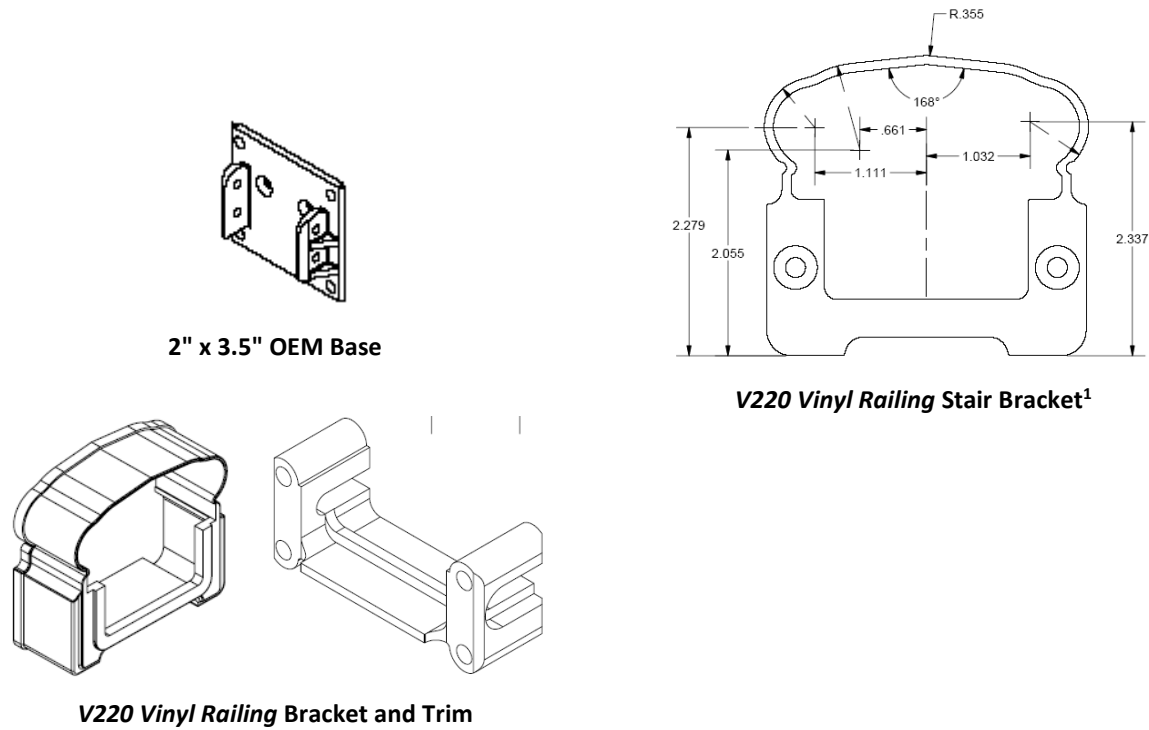
FIGURE 7 - PLASTIC BRACKETS
