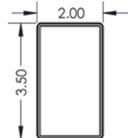
2" x 3 1/2" V310 Bottom Rail Profile
